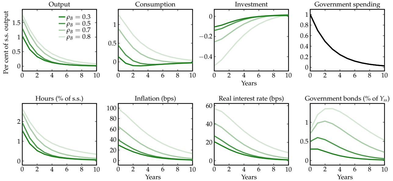
Figure 5: Response to a government spending shock in the quantitative HA-illiq model
